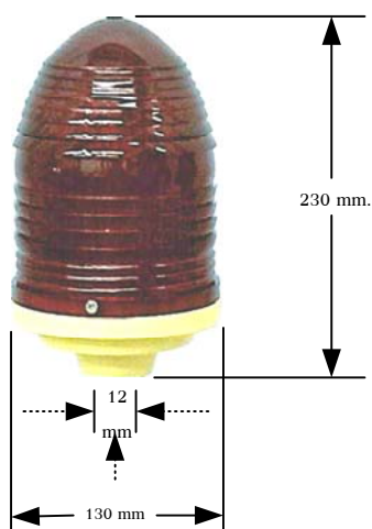
Single type
