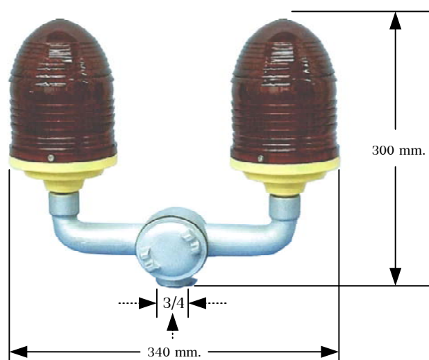
Double type
